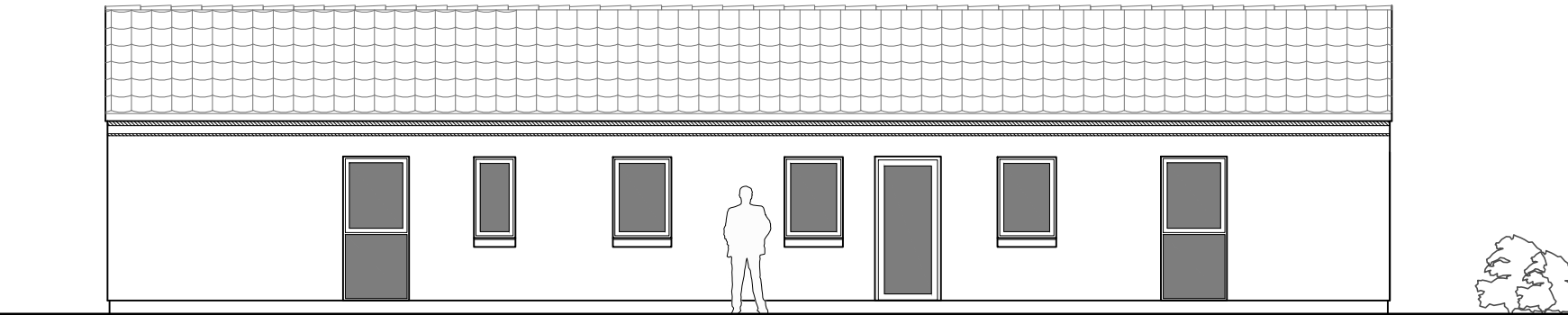
Facade mod
